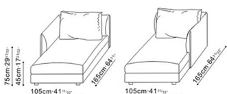
Chaise Section
