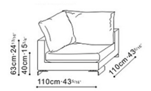
Corner Section
